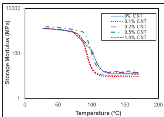
Figure 4: Storage modulus for epoxy and nanocomposites.
