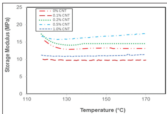
Figure 5: Rubbery modulus for epoxy and nanocomposites.
